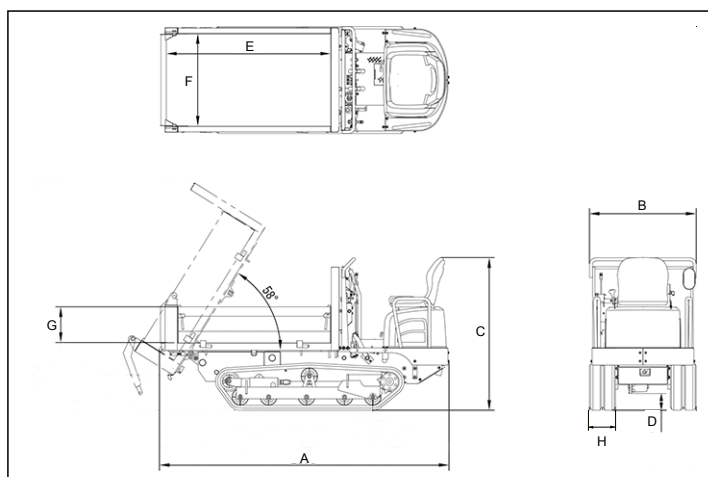
C12R-B
